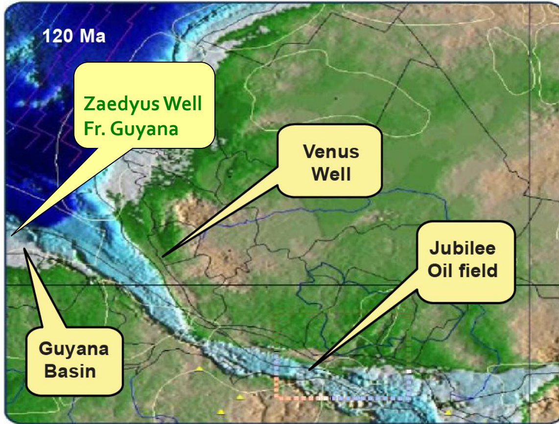
EARLY CRETACEOUS RECONSTRUCTION OF NORTH-WESTERN AFRICA AND SOUTH AMERICA. AFTER TULLOW, 2008.
